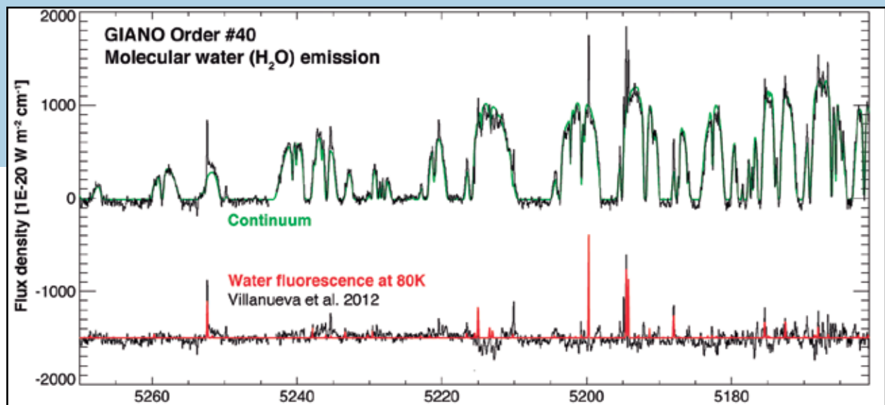
The Figure above shows the water emission for the Lovejoy comet.
